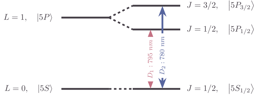
FIGURE VII .2 – Structure fine (transitions D1 et D2) de l'atome de Rubidium ^{87}\text{Rb} .
